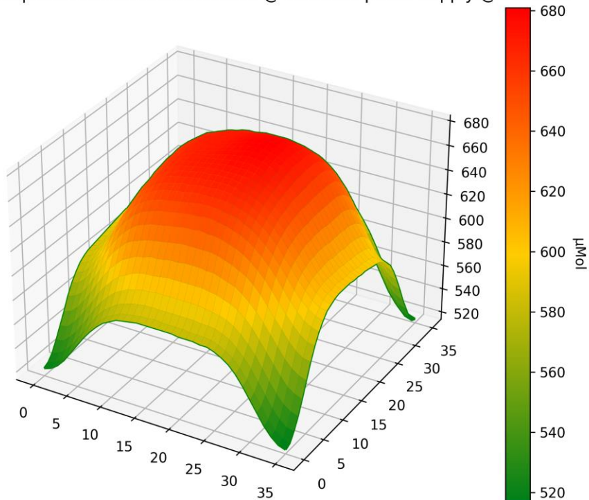
PPFD 3D Heatmap LT-3575 - 3000K - Distance @ 600mm - power supply @ 3500mA
