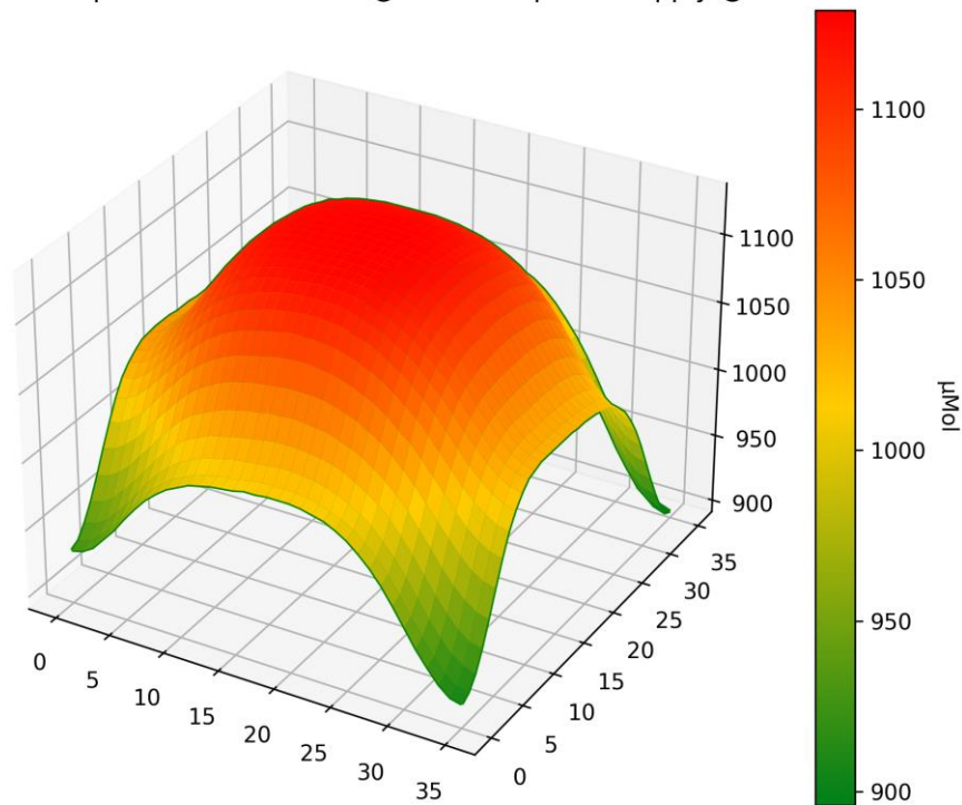
PPFD 3D Heatmap LT-4767 - Distance @ 600mm - power supply @ 5710mA
