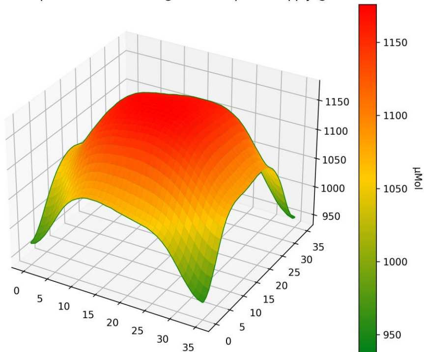
PPFD 3D Heatmap LT-4768 - Distance @ 600mm - power supply @ 5710mA
