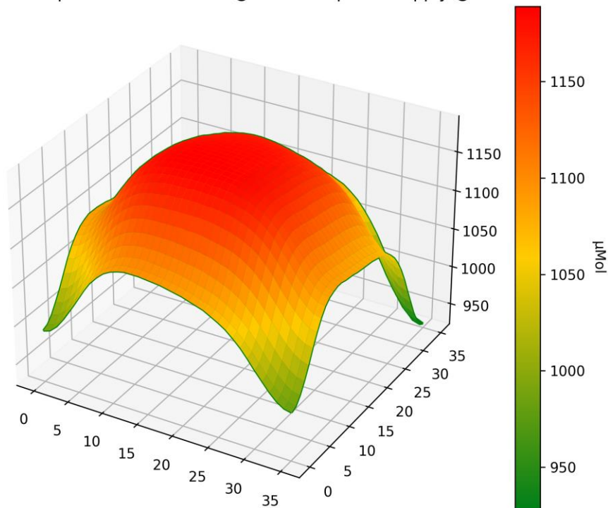
PPFD 3D Heatmap LT-4769 - Distance @ 600mm - power supply @ 5710mA
