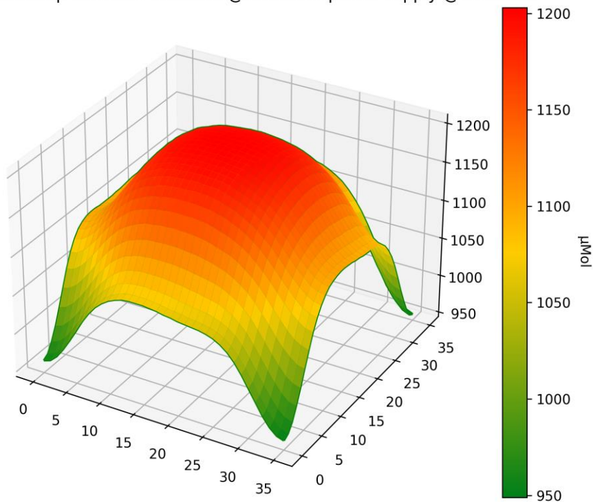
PPFD 3D Heatmap LT-4771 - Distance @ 600mm - power supply @ 5710mA
