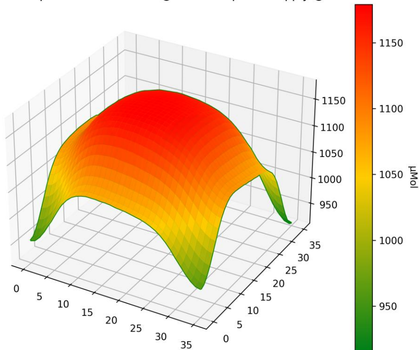
PPFD 3D Heatmap LT-4776 - Distance @ 600mm - power supply @ 5710mA
