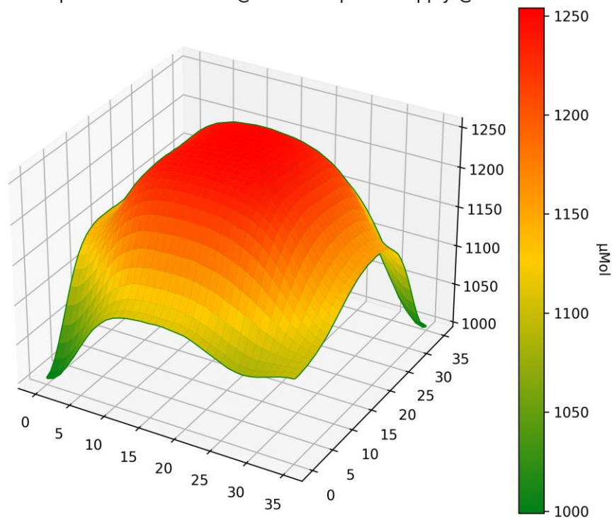
PPFD 3D Heatmap LT-4777 - Distance @ 600mm - power supply @ 5710mA
