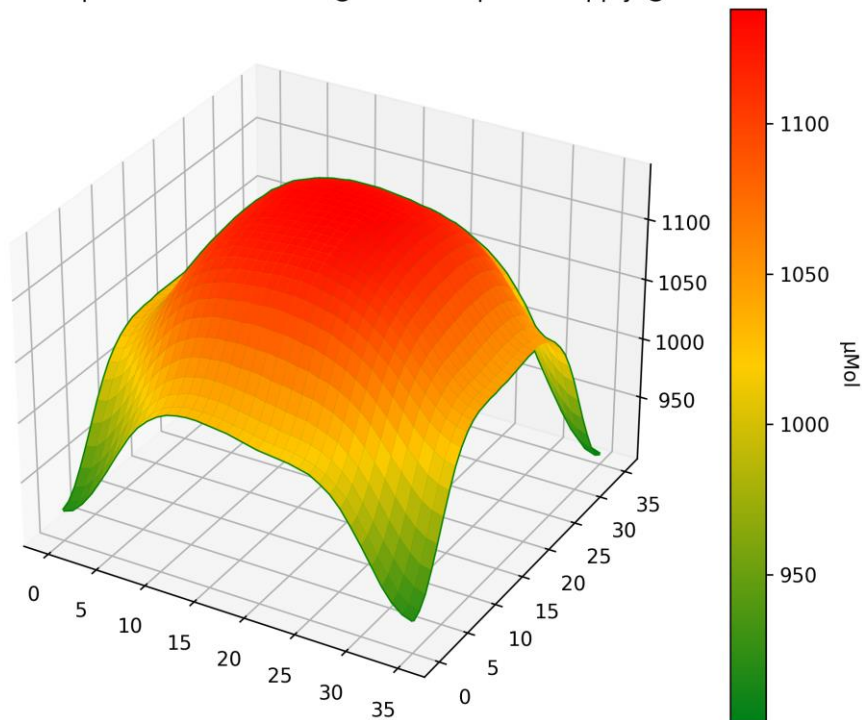
PPFD 3D Heatmap LT-4878 - Distance @ 600mm - power supply @ 5710mA
