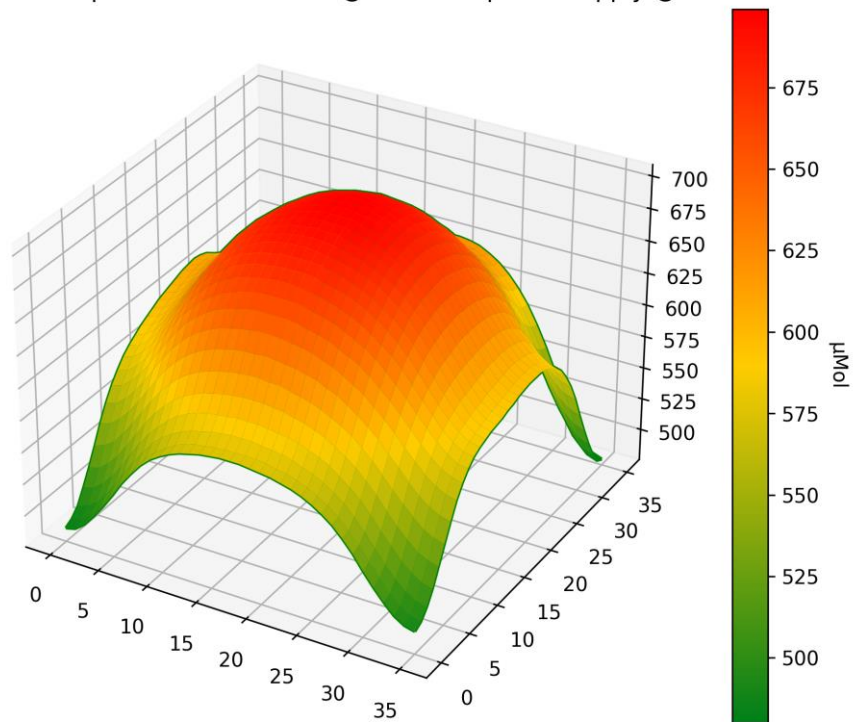
PPFD 3D Heatmap LT-5567 - Distance @ 450mm - power supply @ 700mA
