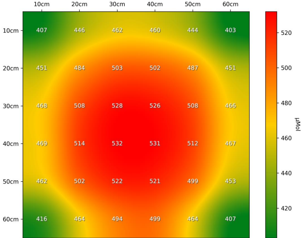
PPFD Heatmap LT-5567 - Distance @ 600mm - power supply @ 700mA
