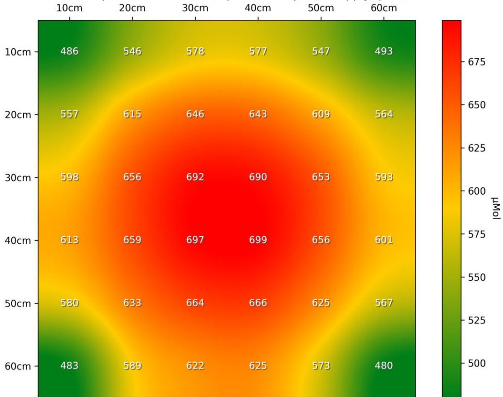
PPFD Heatmap LT-5567 - Distance @ 450mm - power supply @ 700mA
