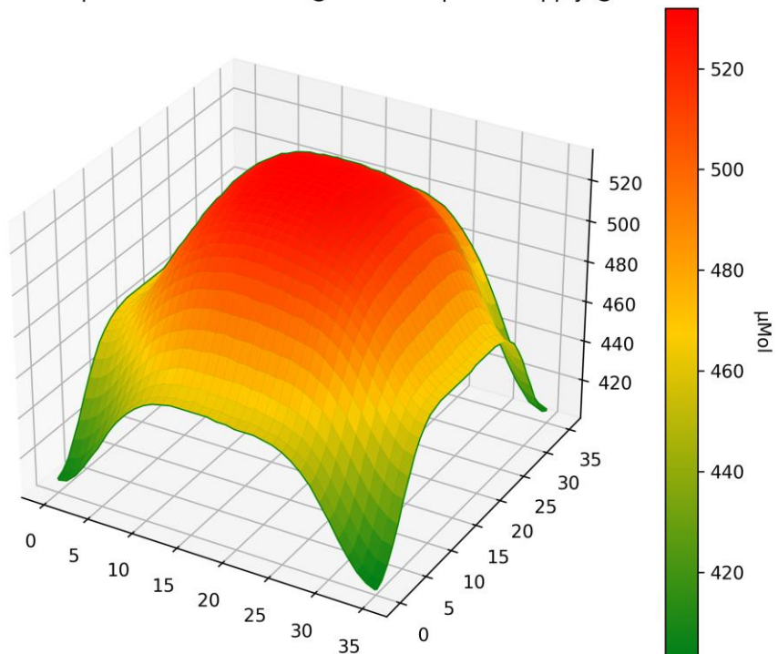
PPFD 3D Heatmap LT-5567 - Distance @ 600mm - power supply @ 700mA
