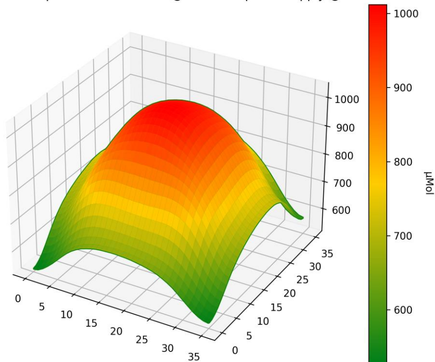
PPFD 3D Heatmap LT-5567 - Distance @ 300mm - power supply @ 700mA
