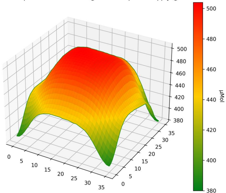
PPFD 3D Heatmap LT-5630 - Distance @ 600mm - power supply @ 700mA
