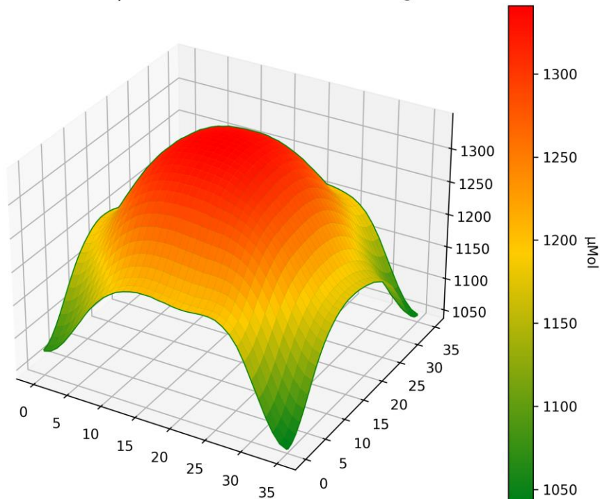
PPFD 3D Heatmap LT-5791 - LIGHTNING Basic RED @600mm
