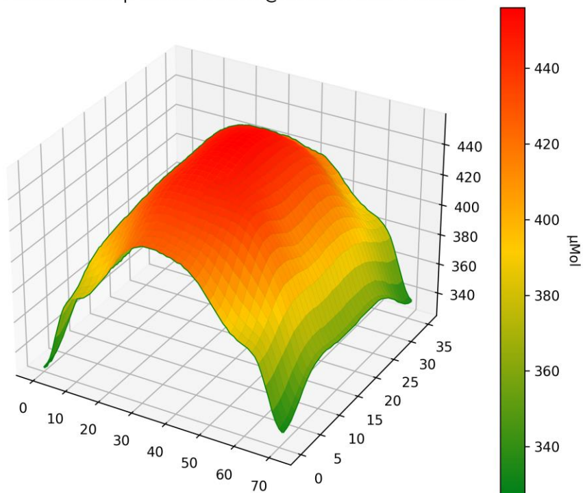
PPFD 3D Heatmap LT-5917 3500K @ 90cm - Power - 100%
