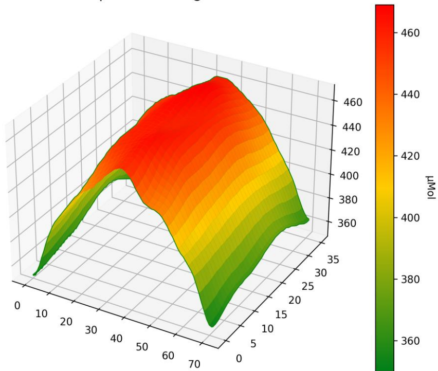
PPFD 3D Heatmap LT-5919 EVO @ 90cm - Power - 100%
