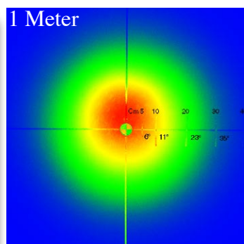
PL121106 (10°) Spectro Metric Analysis
